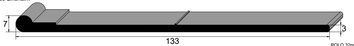
IBC 3794 EPDM 70 Sh A Bandô Linshalm
