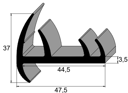
IBC 3595 EPDM 75 Sh A
