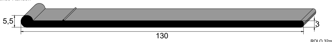
IBC 3466 EPDM 70 Sh A Bandô Linshalm
