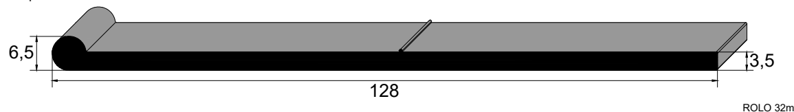
IBC 3610 EPDM 75 Sh A Bandô Randon
